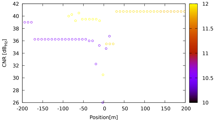
CNR vs position for G32 (L1) on Xiaomi11T - DOY 262 jam. 3
