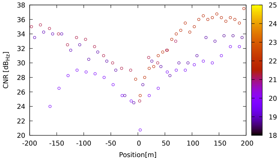
CNR vs position for G32 (L5) on Xiaomi11T - DOY 262 jam. 1
