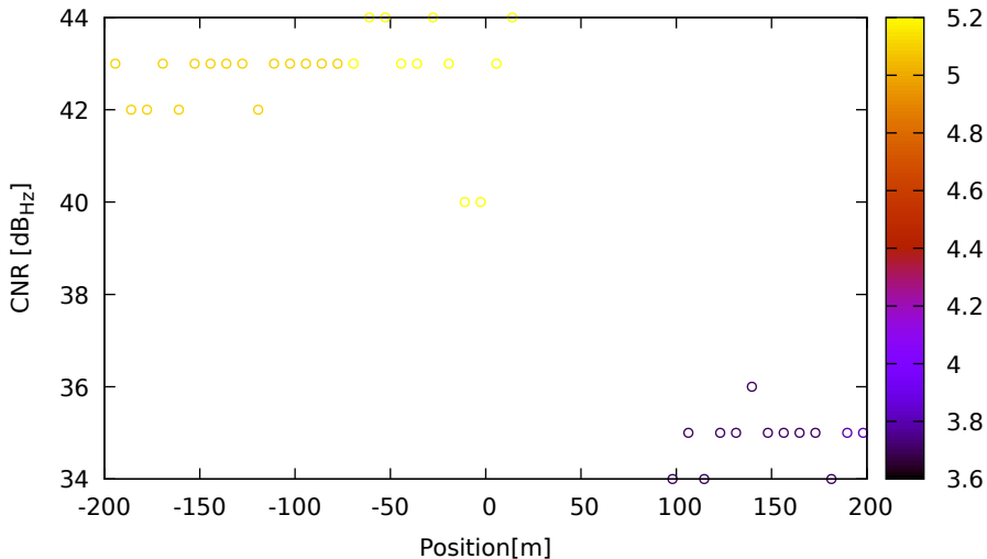
CNR vs position for R02 (G1) on Xiaomi11T - DOY 262 jam. 3
