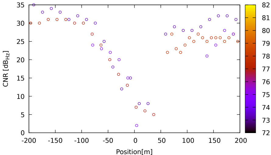
CNR vs position for R08 (G1) on Xiaomi11T - DOY 262 jam. 1
