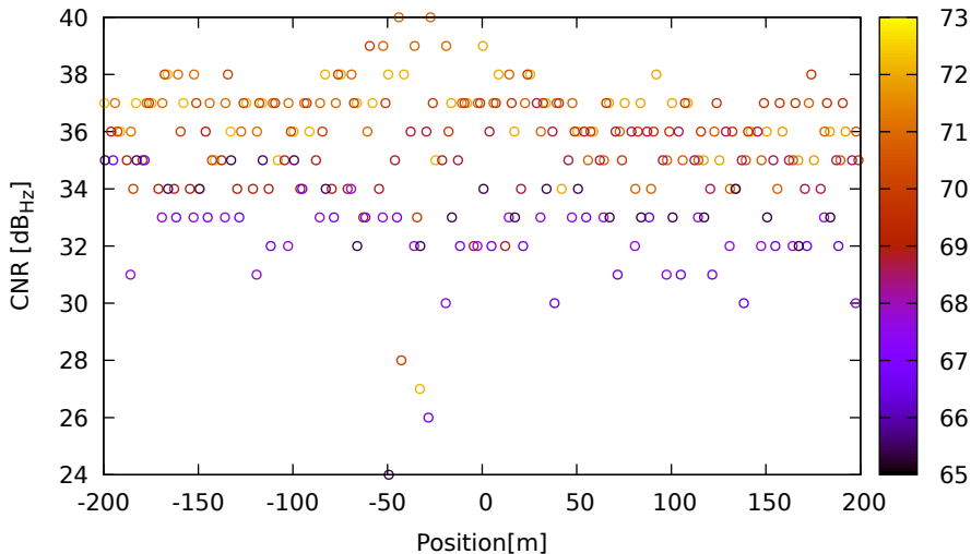
CNR vs position for R08 (G1) on Xiaomi11T - DOY 262 jam. 2
