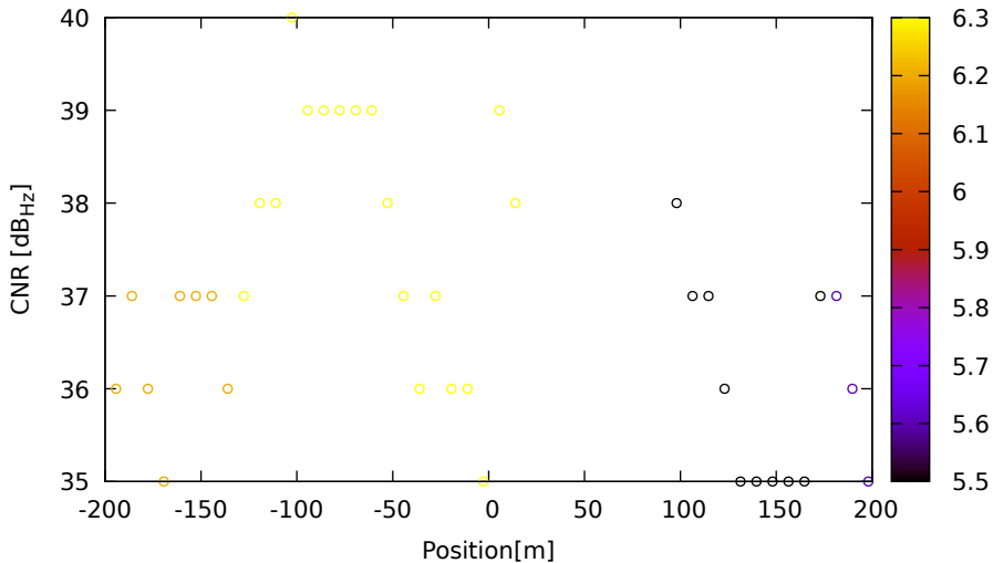
CNR vs position for R09 (G1) on Xiaomi11T - DOY 262 jam. 3
