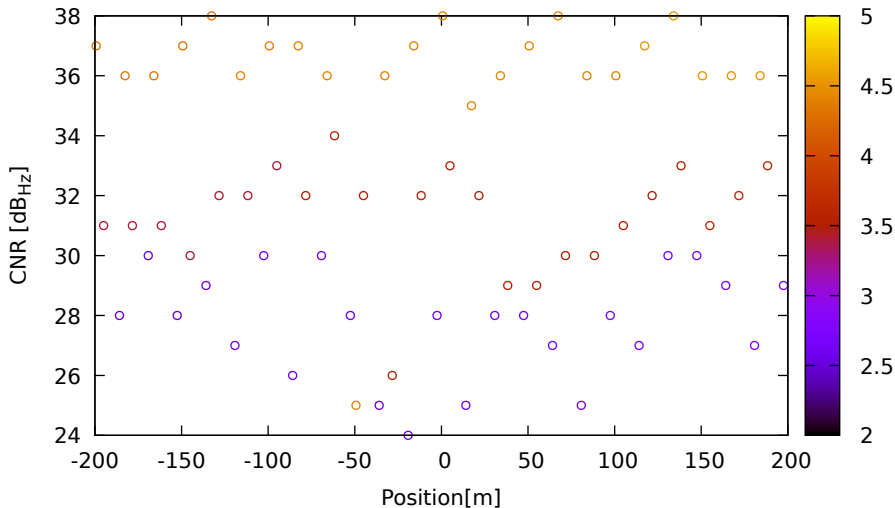
CNR vs position for R17 (G1) on Xiaomi11T - DOY 262 jam. 2
