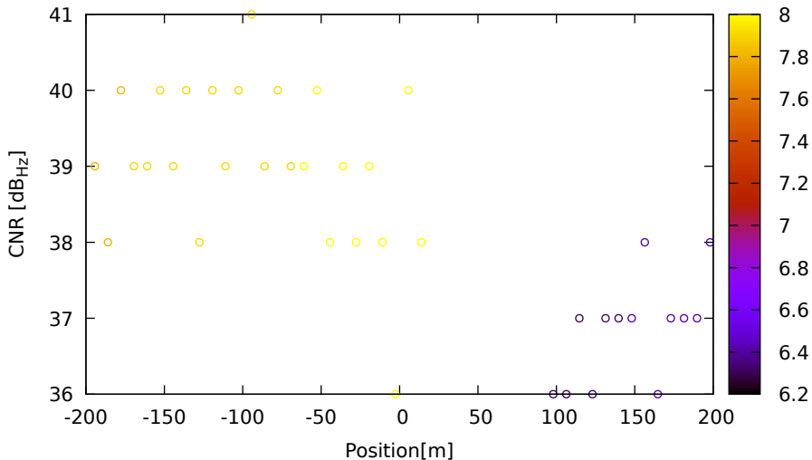
CNR vs position for R17 (G1) on Xiaomi11T - DOY 262 jam. 3
