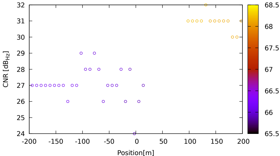
CNR vs position for R23 (G1) on Xiaomi11T - DOY 262 jam. 3
