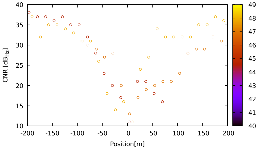
CNR vs position for R24 (G1) on Xiaomi11T - DOY 262 jam. 1
