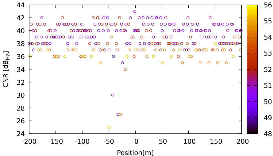
CNR vs position for R24 (G1) on Xiaomi11T - DOY 262 jam. 2
