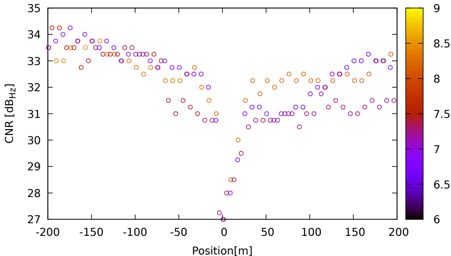
CNR vs position for C11 (B1) on XiaomiMi8 - DOY 262 jam. 3
