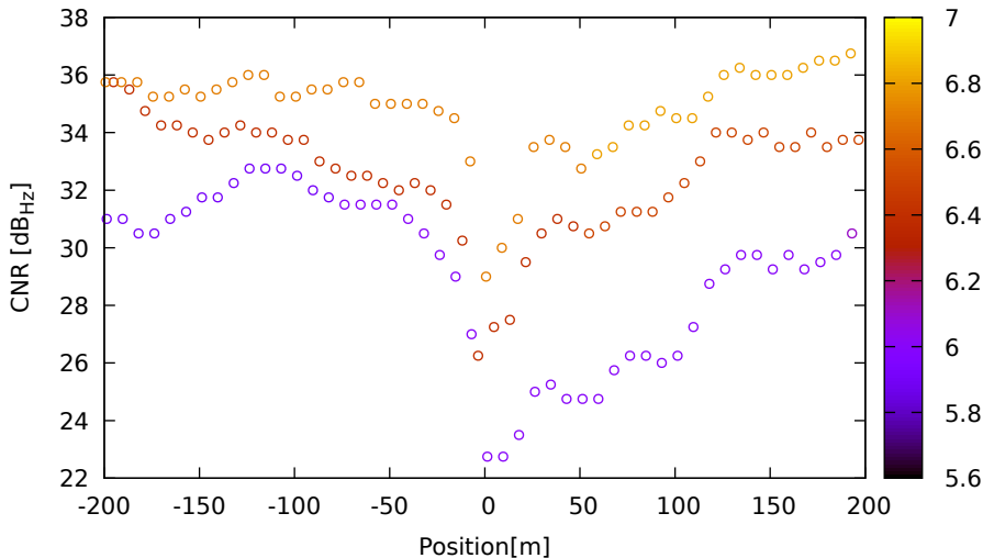
CNR vs position for C26 (B1) on XiaomiMi8 - DOY 262 jam. 3
