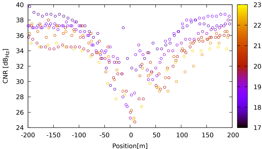
CNR vs position for C27 (B1) on XiaomiMi8 - DOY 262 jam. 1
