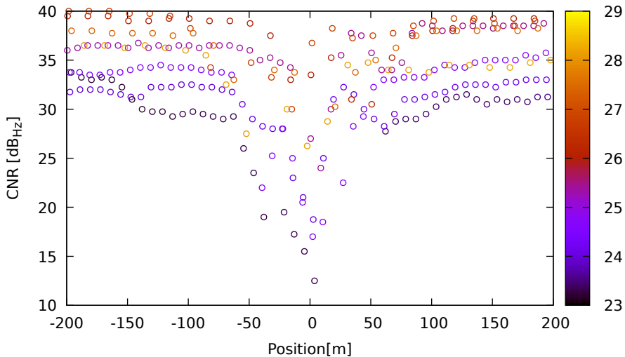
CNR vs position for C27 (B1) on XiaomiMi8 - DOY 262 jam. 2
