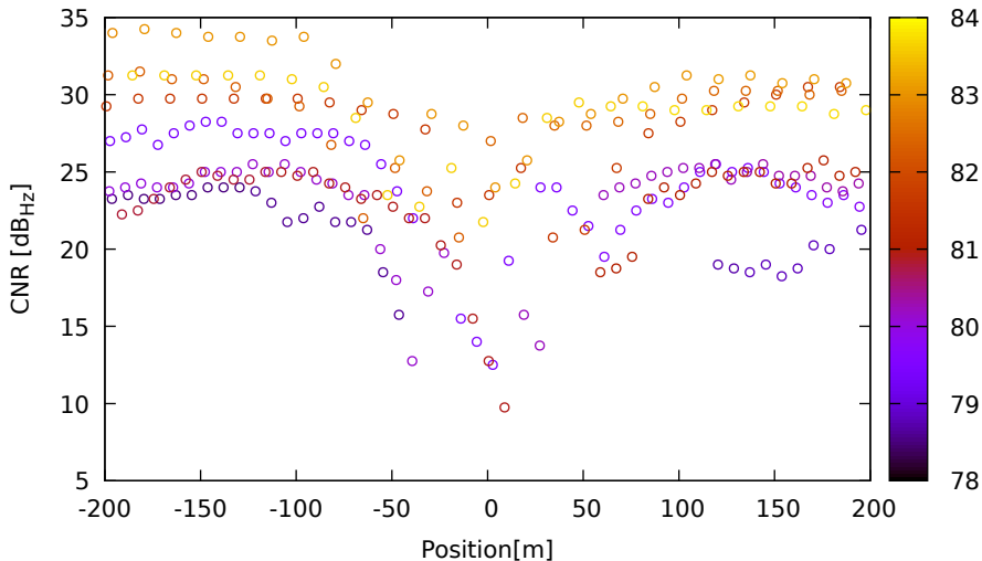
CNR vs position for C33 (B1) on XiaomiMi8 - DOY 262 jam. 2
