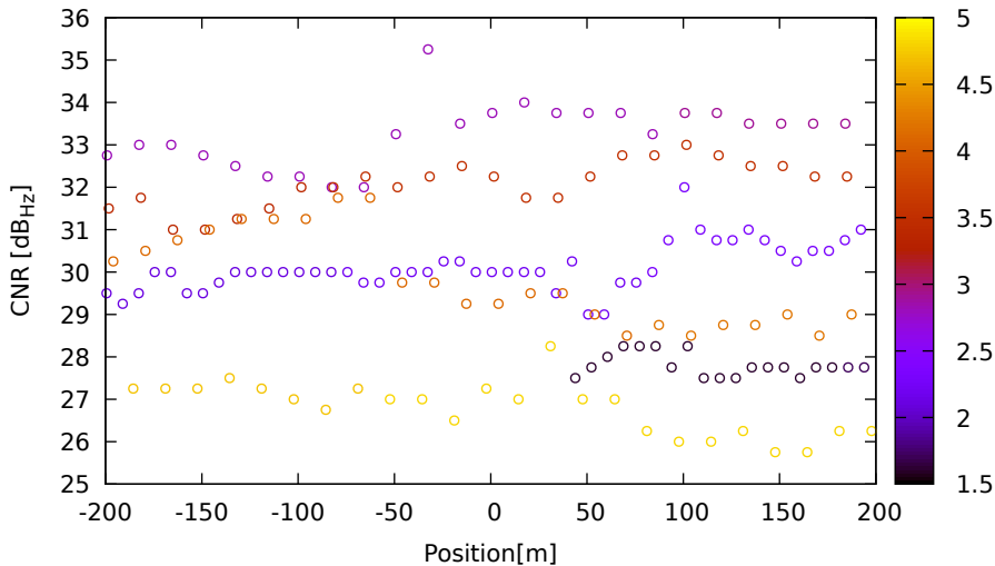
CNR vs position for E03 (E5a) on XiaomiMi8 - DOY 262 jam. 2
