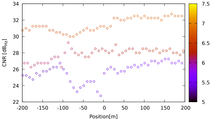
CNR vs position for E03 (E5a) on XiaomiMi8 - DOY 262 jam. 3
