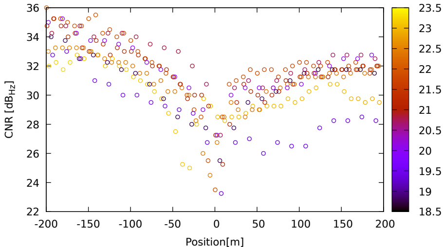
CNR vs position for E04 (E1) on XiaomiMi8 - DOY 262 jam. 1
