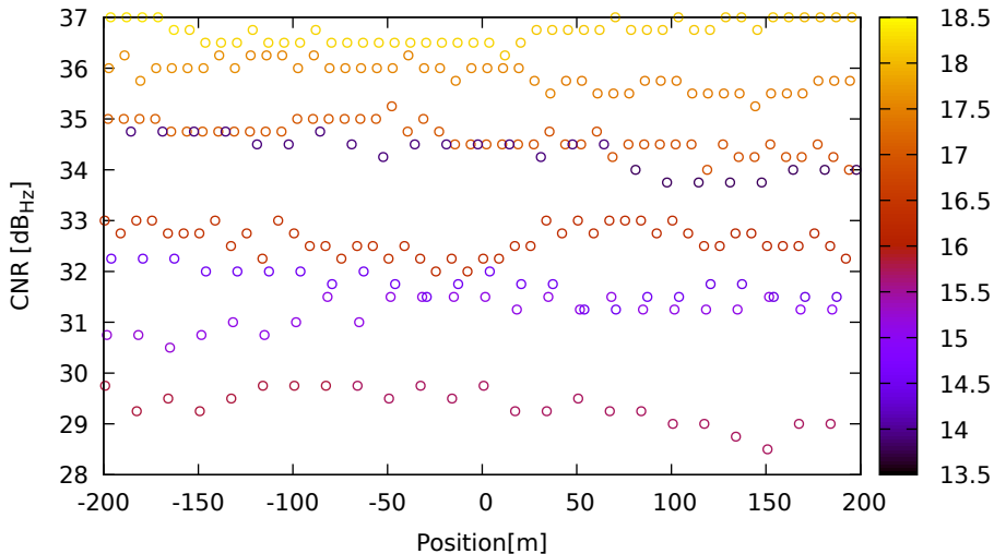
CNR vs position for E04 (E5a) on XiaomiMi8 - DOY 262 jam. 2
