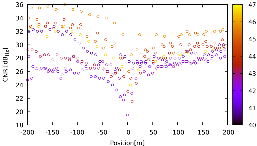
CNR vs position for E05 (E1) on XiaomiMi8 - DOY 262 jam. 1
