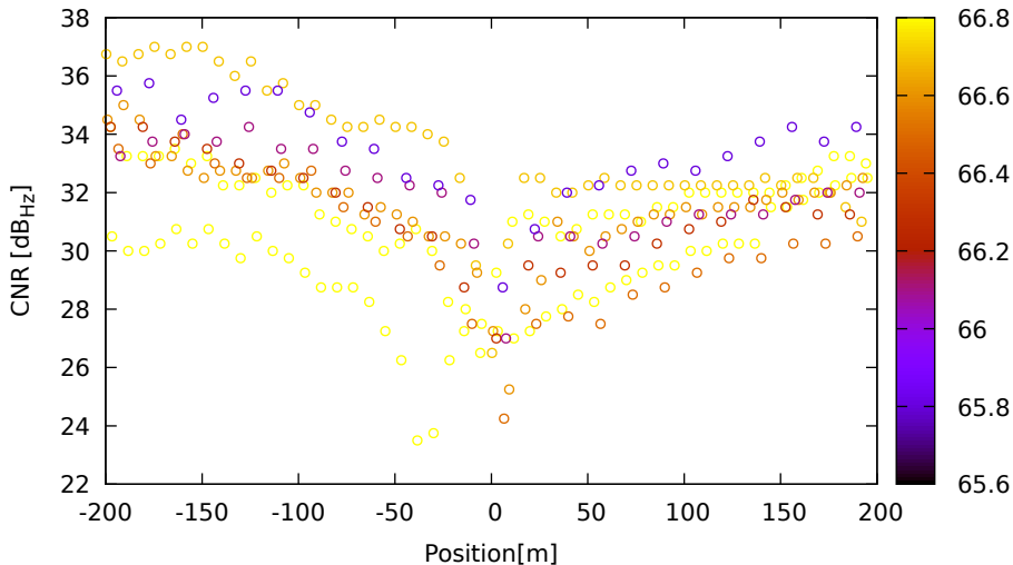
CNR vs position for E09 (E1) on XiaomiMi8 - DOY 262 jam. 1
