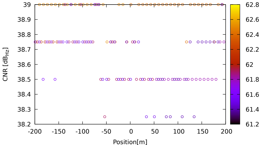
CNR vs position for E09 (E5a) on XiaomiMi8 - DOY 262 jam. 3
