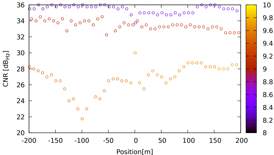
CNR vs position for E15 (E5a) on XiaomiMi8 - DOY 262 jam. 3
