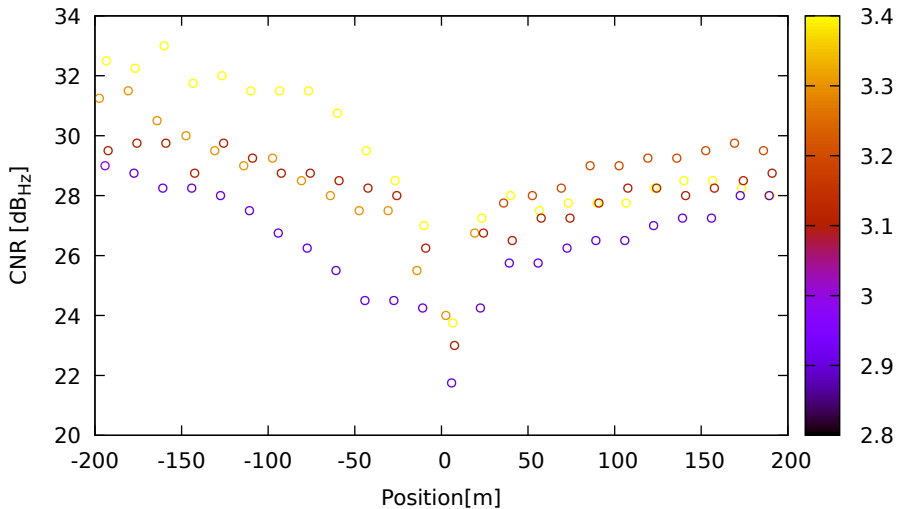
CNR vs position for E27 (E1) on XiaomiMi8 - DOY 262 jam. 1
