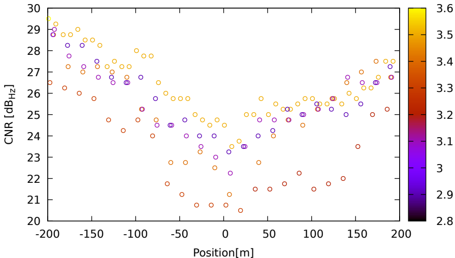
CNR vs position for E27 (E5a) on XiaomiMi8 - DOY 262 jam. 1
