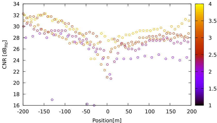
CNR vs position for E30 (E1) on XiaomiMi8 - DOY 262 jam. 1
