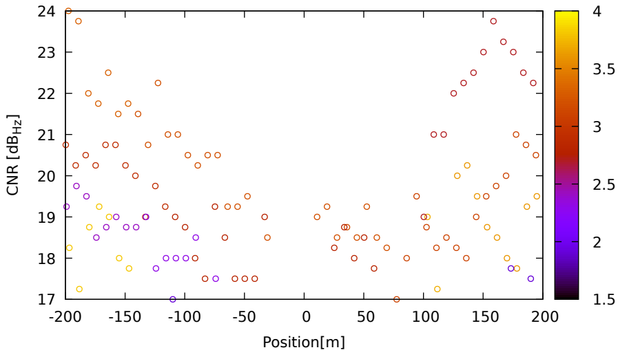
CNR vs position for E30 (E5a) on XiaomiMi8 - DOY 262 jam. 1
