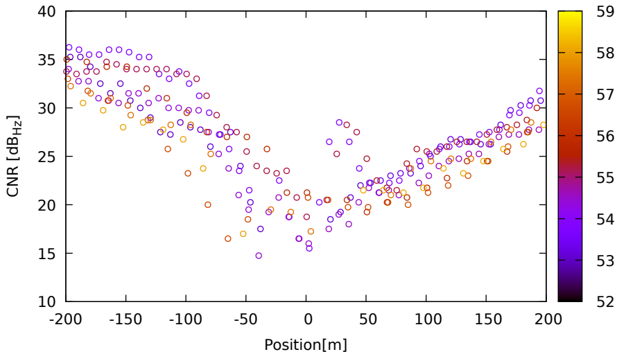
CNR vs position for E34 (E1) on XiaomiMi8 - DOY 262 jam. 2
