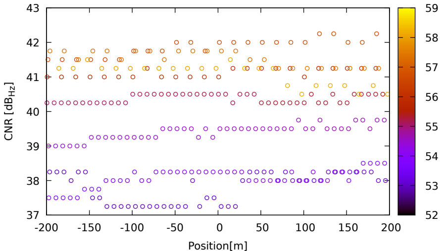
CNR vs position for E34 (E5a) on XiaomiMi8 - DOY 262 jam. 2
