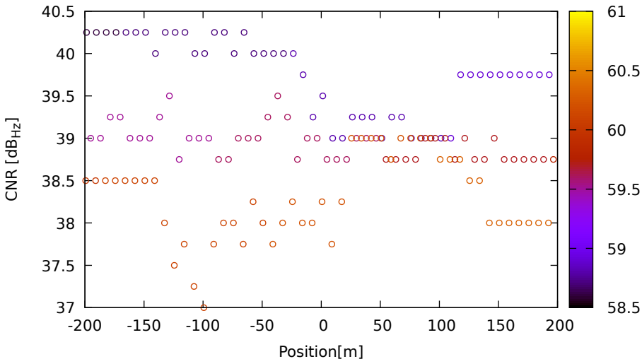
CNR vs position for E34 (E5a) on XiaomiMi8 - DOY 262 jam. 3
