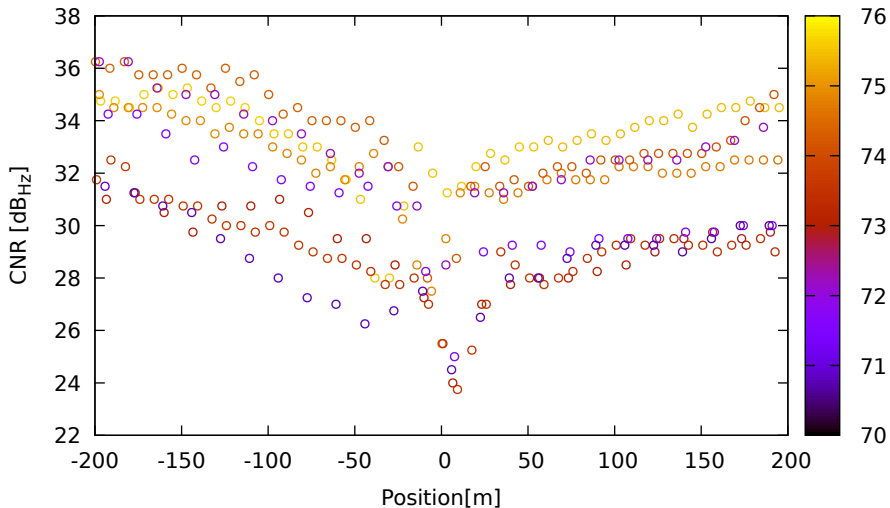
CNR vs position for E36 (E1) on XiaomiMi8 - DOY 262 jam. 1
