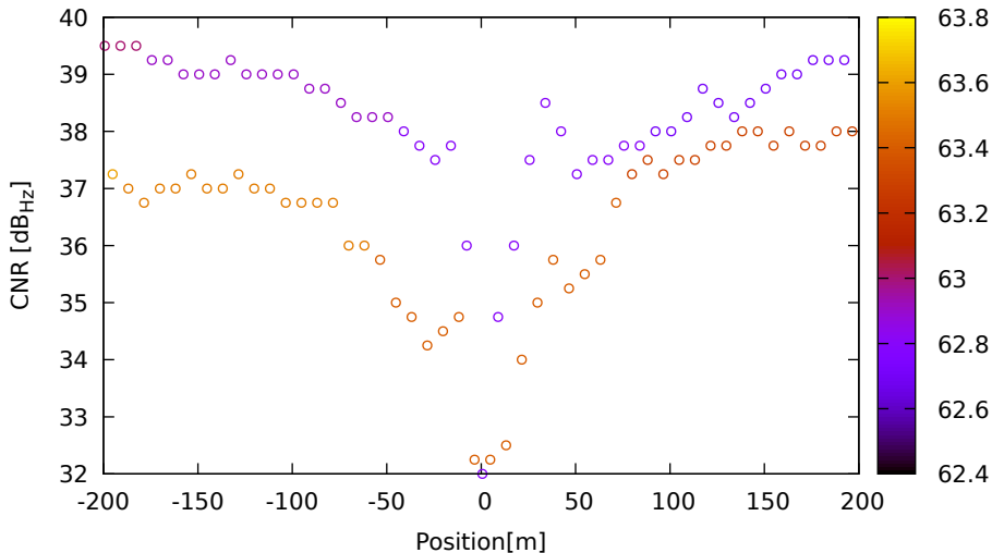
CNR vs position for E36 (E1) on XiaomiMi8 - DOY 262 jam. 3
