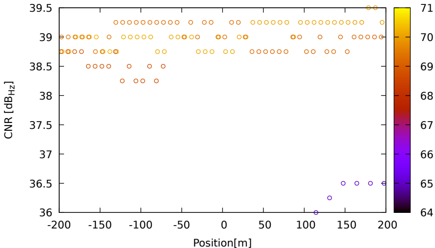
CNR vs position for E36 (E5a) on XiaomiMi8 - DOY 262 jam. 2
