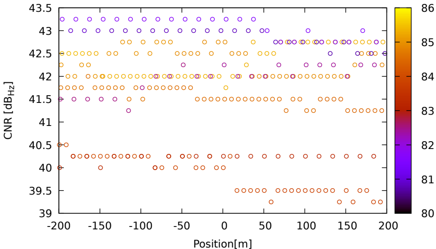
CNR vs position for G01 (L5) on XiaomiMi8 - DOY 262 jam. 2
