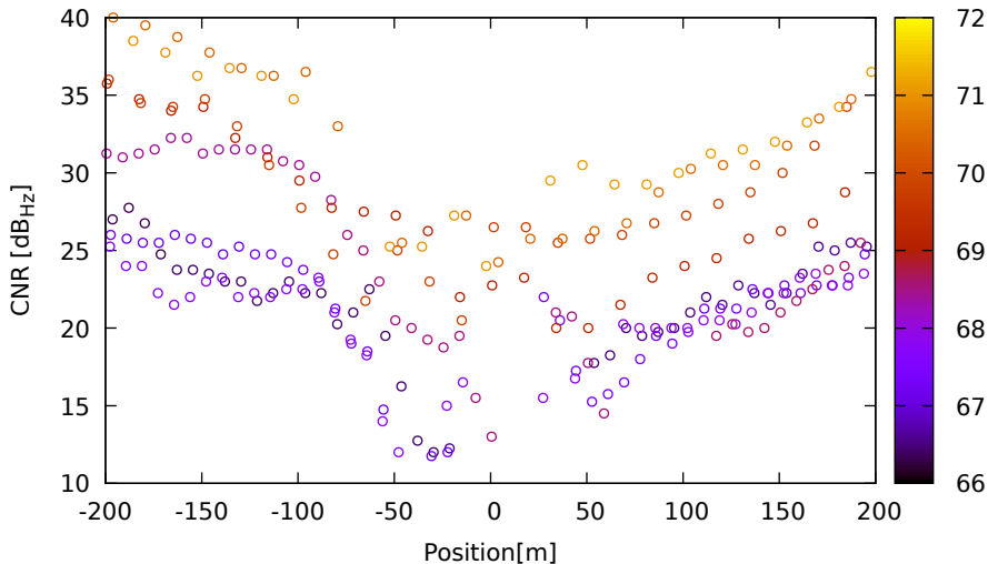
CNR vs position for G03 (L1) on XiaomiMi8 - DOY 262 jam. 2
