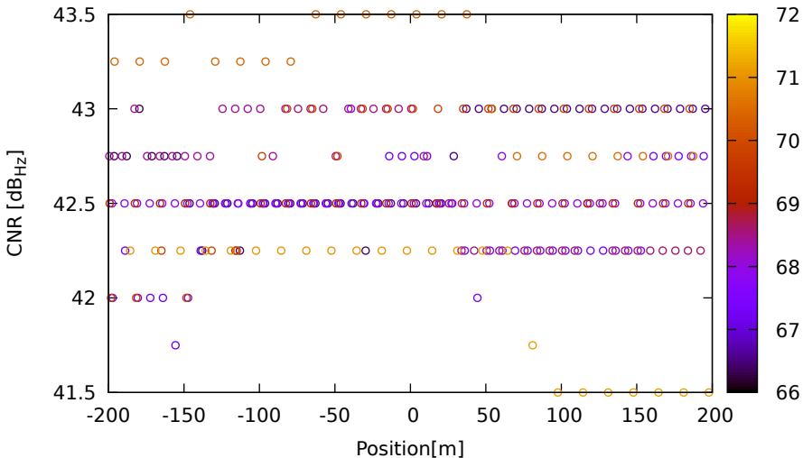
CNR vs position for G03 (L5) on XiaomiMi8 - DOY 262 jam. 2
