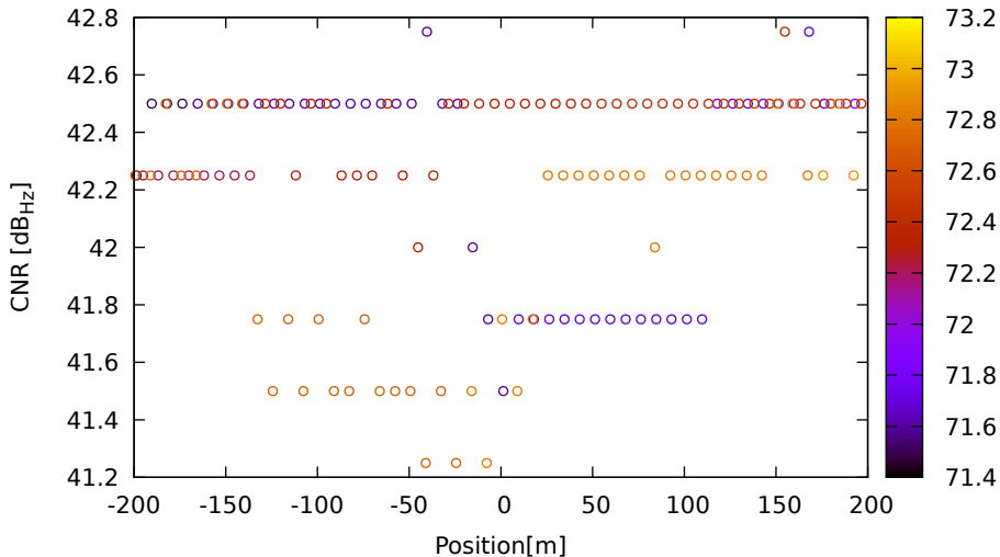
CNR vs position for G03 (L5) on XiaomiMi8 - DOY 262 jam. 3
