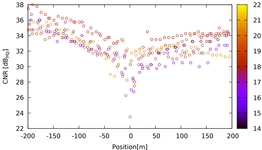
CNR vs position for G08 (L1) on XiaomiMi8 - DOY 262 jam. 1
