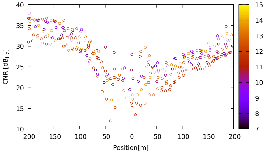
CNR vs position for G08 (L1) on XiaomiMi8 - DOY 262 jam. 2
