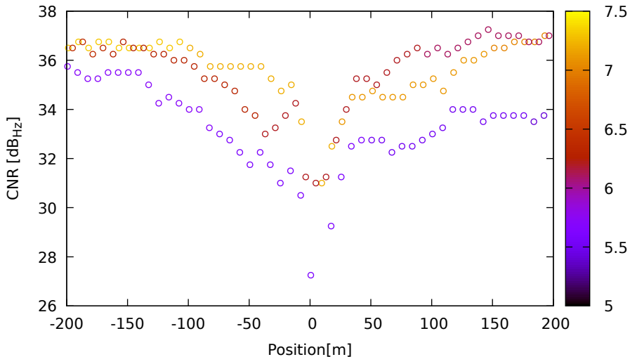
CNR vs position for G08 (L1) on XiaomiMi8 - DOY 262 jam. 3
