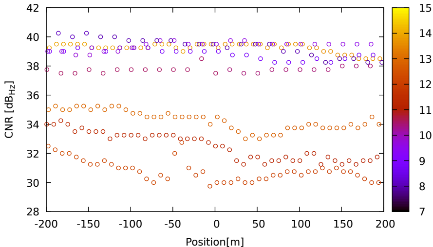
CNR vs position for G08 (L5) on XiaomiMi8 - DOY 262 jam. 2
