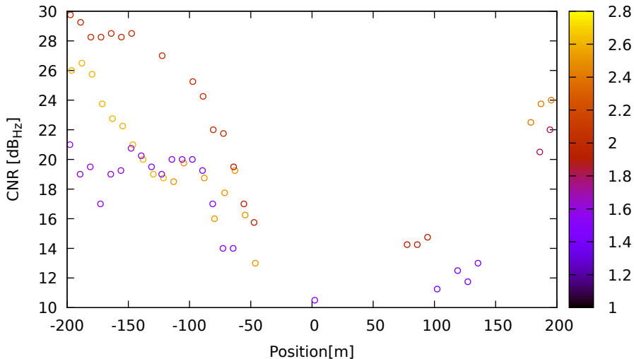
CNR vs position for G14 (L1) on XiaomiMi8 - DOY 262 jam. 2
