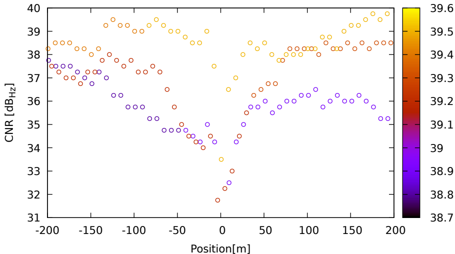
CNR vs position for G17 (L1) on XiaomiMi8 - DOY 262 jam. 3
