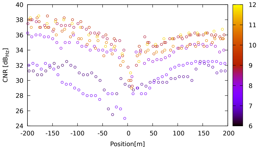
CNR vs position for G19 (L1) on XiaomiMi8 - DOY 262 jam. 1
