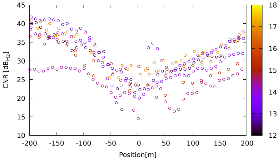
CNR vs position for G19 (L1) on XiaomiMi8 - DOY 262 jam. 2
