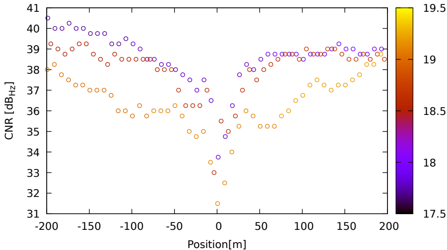
CNR vs position for G19 (L1) on XiaomiMi8 - DOY 262 jam. 3
