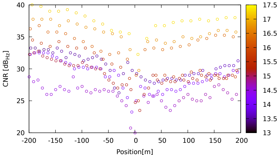
CNR vs position for G31 (L1) on XiaomiMi8 - DOY 262 jam. 1
