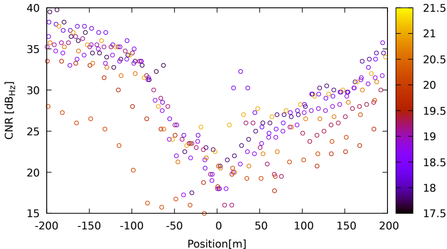
CNR vs position for G31 (L1) on XiaomiMi8 - DOY 262 jam. 2
