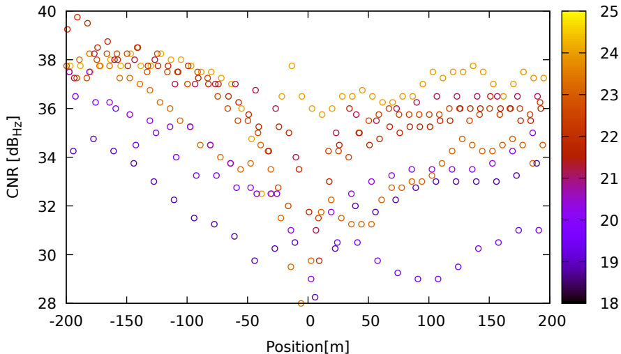
CNR vs position for G32 (L1) on XiaomiMi8 - DOY 262 jam. 1
